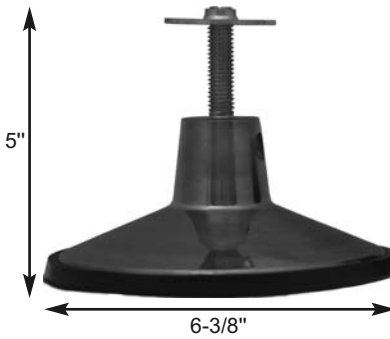
B0533 Polished Cast Aluminum W/Rubber Trim. Bolt Dia. Is 1/2" x 13 Includes Nut (B0535)
