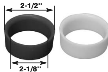
Hole Liners For 2-1/8" Balls B0066 – Red B0067 – White
