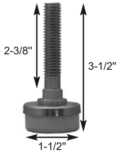
B0534 Heavy-Duty Rigid W/Rubber Base Bolt Dia. Is 1/2" x 13
