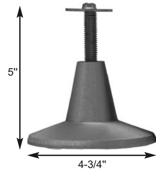
B3018 Solid Brushed Aluminum. Bolt Dia. Is 1/2" x 13 Includes Nut (B0535)
